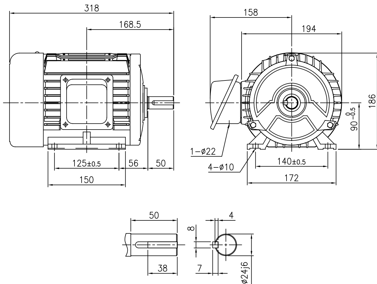
SHAFT EXTENSION
